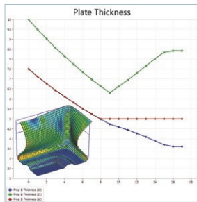
Optimization
